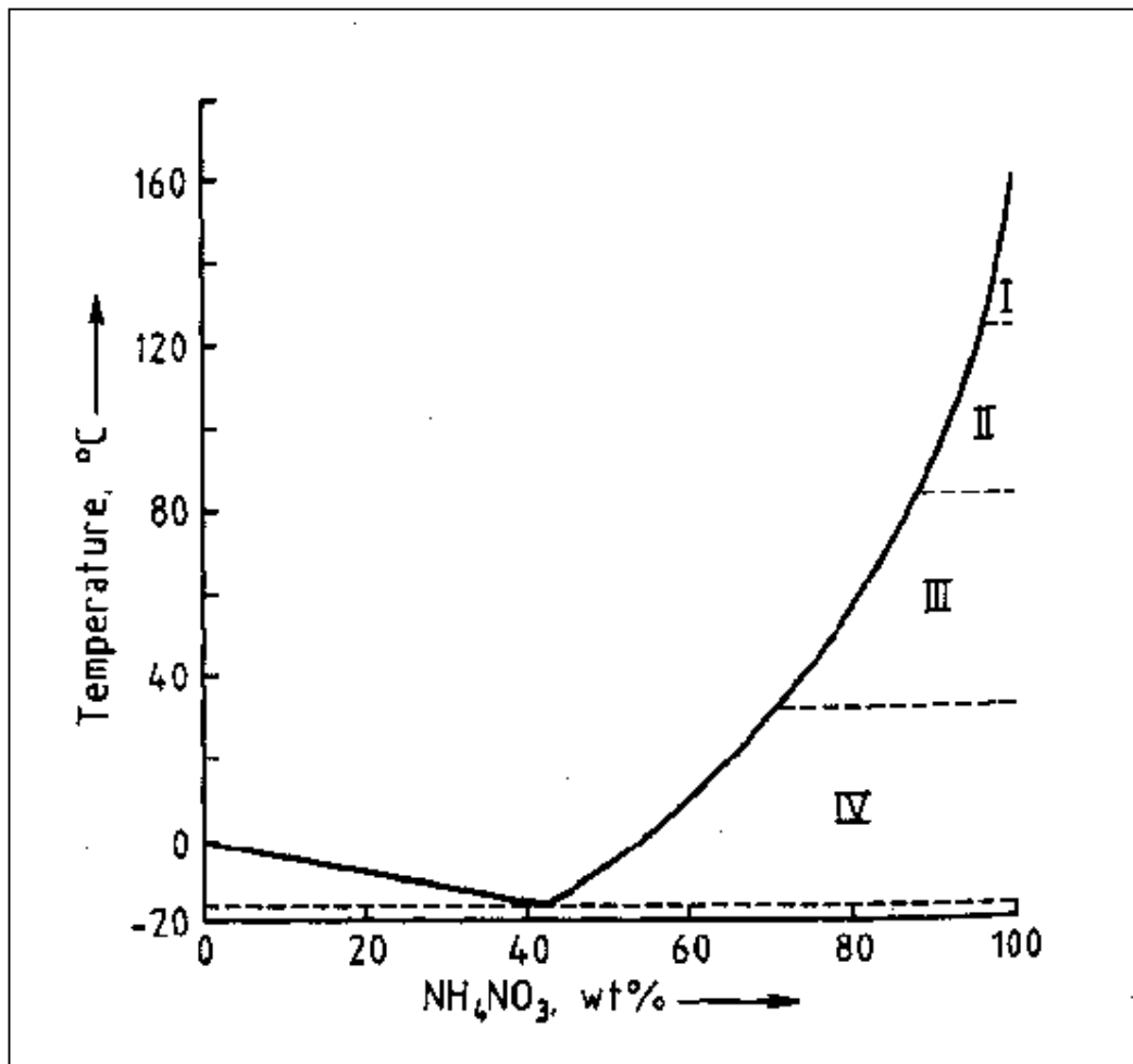
Figure 12. The solubility of ammonium nitrate in water (weight% on x-axis) versus the temperature ( ^{\circ}\text{C} ). Ammonium nitrate has 5 modifications: I: cubic, II tetragonal: III: orthorhombic, IV: orthorhombic and V tetragonal. Very concentrated ammonium nitrate solutions can be formed well above the boiling point of water.
