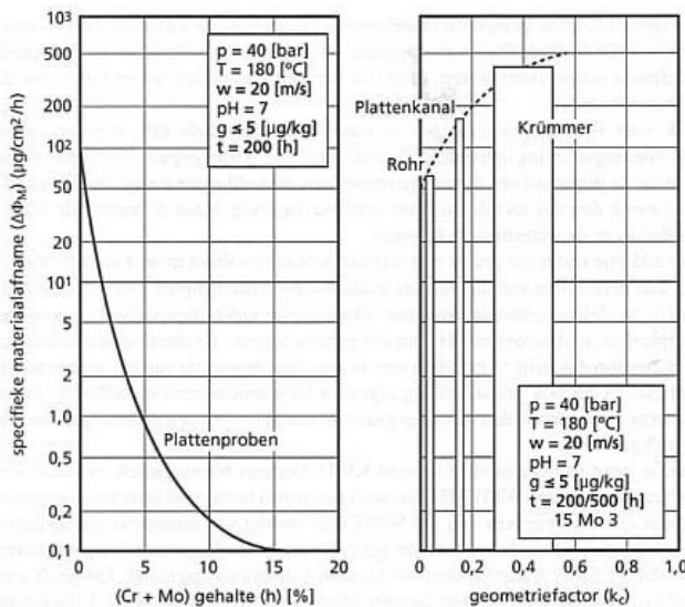
Figure 3. Influence of Cr+Mo content and the geometry on erosion corrosion according to the experiments of KWU (Heitmann 1 , 1982).
